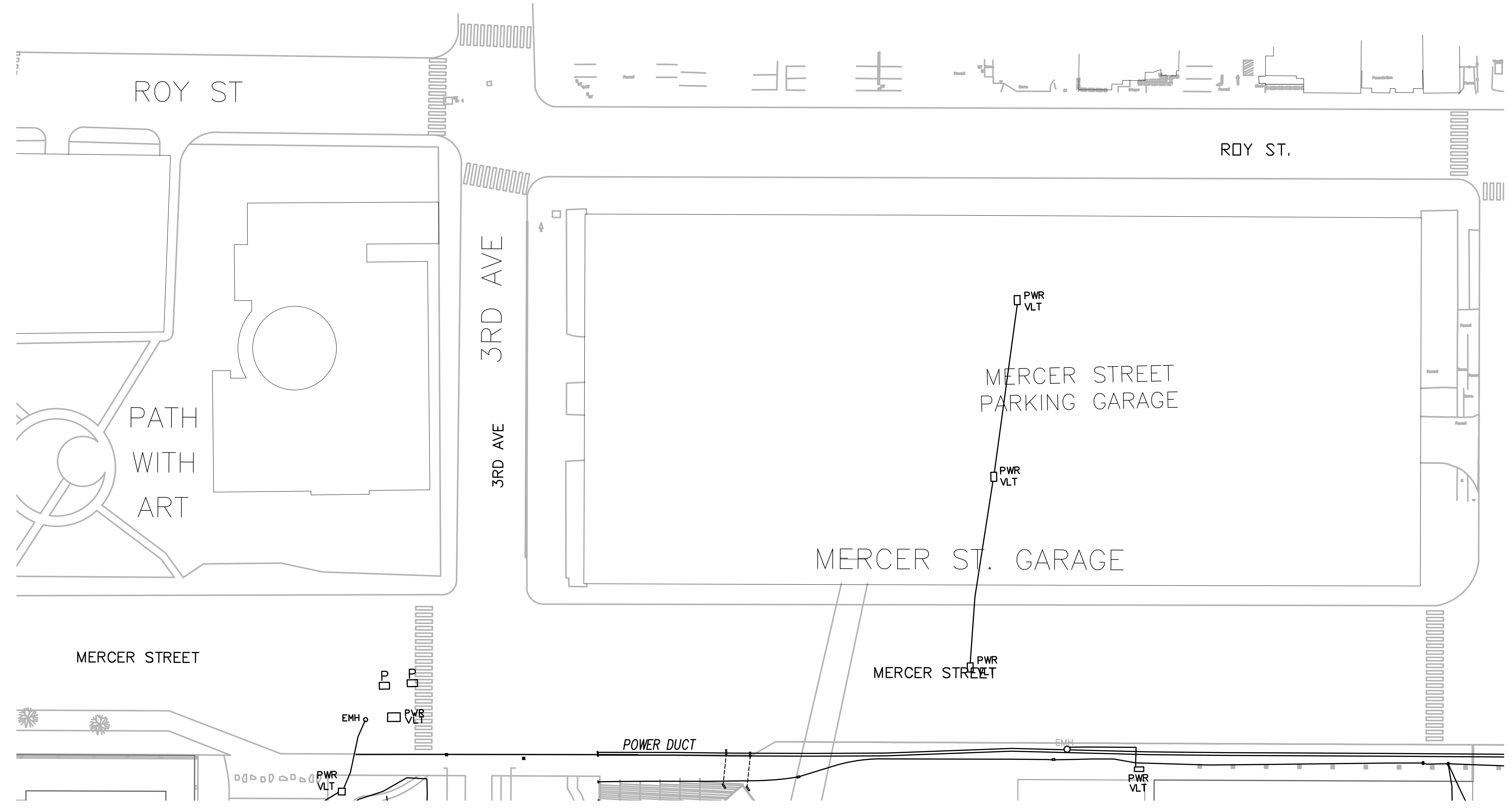
SECTOR PLAN SCALE: 1" = 40'-0"
