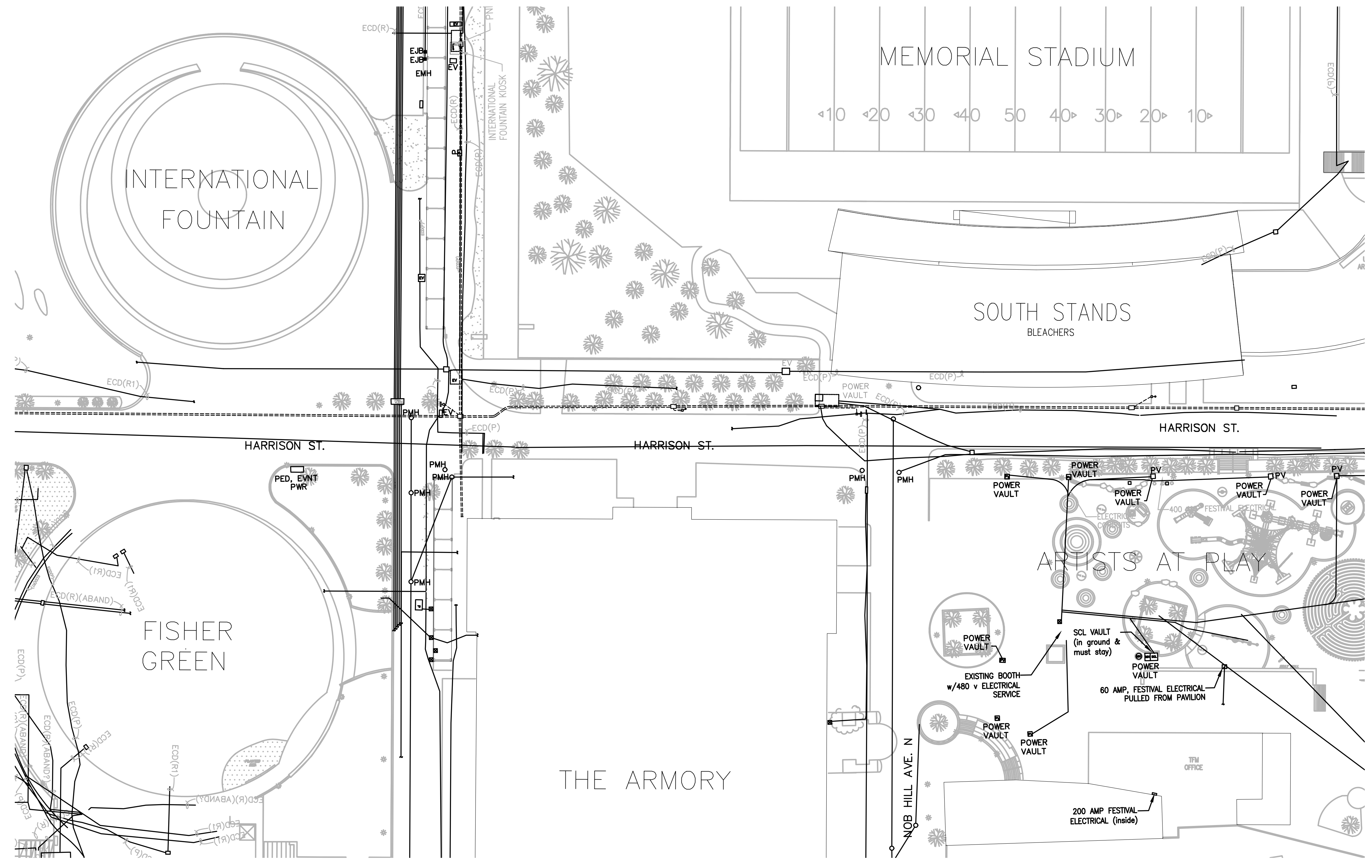
SECTOR PLAN SCALE: 1" = 40'-0"
